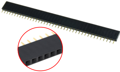
◆ 40 PINES PITCH 2.54mm
