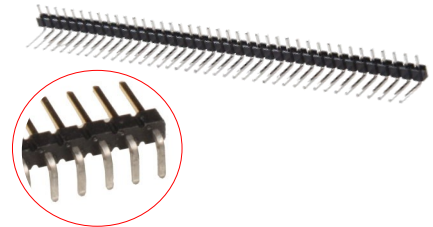
◆ 40 PINES CURVOS PITCH 2.54mm
