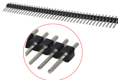
◆ 40 PINES PITCH 2.54mm
